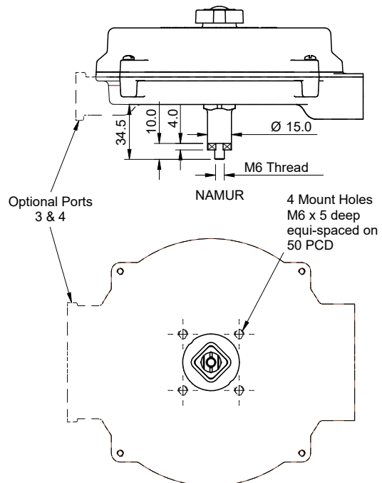
12, 14 & 15 DIRECT MOUNT OPTION ADDITIONAL ADAPTOR WEIGHT: 0.56 kg
