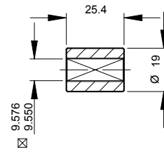
Standard Coupling (supplied with actuator weight 0.09 lbs/0.04 kg)
